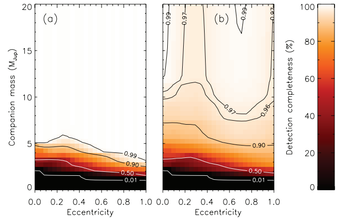
Figure 4. Probability of at least one 5\sigma detection of a companion with a 6.3 year orbit around Sirius A in our three data sets, as a function of companion mass m and eccentricity e . (a) The case of coplanar orbits with the Sirius AB system (inclination i = 136.6 ). All companions above 6 M_{\text{Jup}} can be rejected regardless of orbital phase (100% completeness). The completeness remains above 50% down to 2\text{--}3.5 M_{\text{Jup}} depending on eccentricity. (b) If the inclination is unconstrained ( p(i) \propto \sin i ), edge-on orbits become possible, introducing a chance of a few percent that Sirius C might elude detection in all observations. Nevertheless, our three data sets provide decisive evidence against the existence of Sirius C as proposed by Benest & Duvent (1995).
