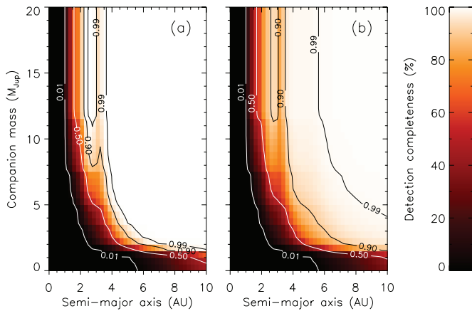
Figure 5. Probability of at least one 5\sigma detection of a companion around Sirius A in our three data sets, as a function of companion mass m and semimajor axis a . A flat distribution in eccentricities is assumed. (a) The case of coplanar orbits with the Sirius AB system (inclination i = 136.6^\circ ). (b) The case of unconstrained inclination ( p(i) \propto \sin i ). The false negative probability is large for the stable planet orbit regime at a \lesssim 2.17 (Holman & Wiegert 1999).
