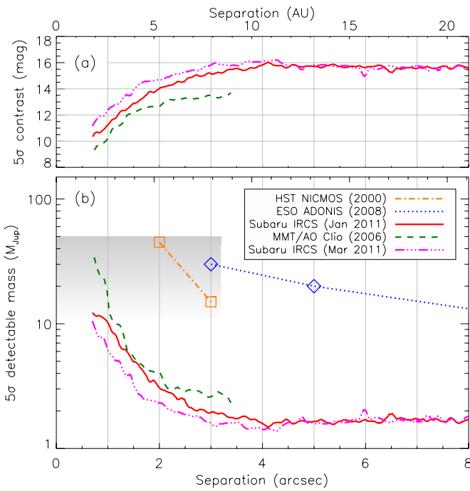
Figure 3. Limits on faint companions to Sirius A. (a) Effective 5\sigma detectable contrast to Sirius A in the 2011 January \text{Br } \alpha data, (solid red), the M -band data (dashed green), and the 2011 March \text{Br } \alpha data (dash-dot-dot-dotted magenta) as a function of separation, corrected for partial subtraction. (b) The companion masses corresponding to those contrasts, derived according to an updated version of the method of Janson et al. (2008) from the COND evolutionary model (Allard et al. 2001; Baraffe et al. 2003). For comparison, the constraints established by Kuchner & Brown (2000, dash-dotted orange) and Bonnet-Bidaud & Pantin (2008, dotted blue) are overplotted. The gray shaded area indicates the parameter space of a \lesssim 50 M_{\text{Jup}} companion in a 6.3 year orbit (semimajor axis a = 1'6 ). (A color version of this figure is available in the online journal.)
