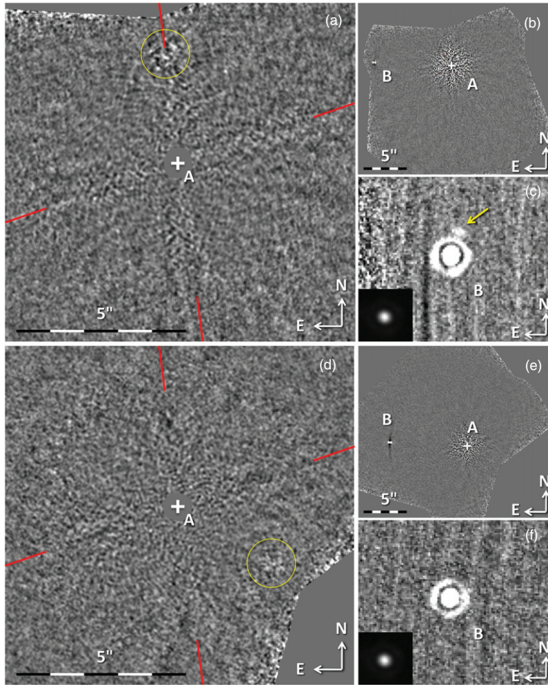
Figure 1. (a–c) Results of the 2011 January ADI observations of the Sirius system in the Br \alpha band with Subaru IRCS. (a) Signal-to-noise map of the inner \sim 10'' \times 10'' , calculated in concentric annuli after convolution with a 4 pixel diameter circular aperture. The stretch is [-5\sigma, 5\sigma] . The location of Sirius A is marked with a white plus sign. The short red lines indicate the position angles where residuals of the spider diffraction pattern slightly elevate the noise level. The yellow circle marks the area of increased noise generated by one of the unused mirror holes in the field of view. (b) Full field of view of the ADI intensity image. Sirius B is visible to the east of Sirius A. (c) Non-differential image of Sirius B. Unsharp masking on the scale of 15 pixels ( 3 \lambda/D ) has been applied to reduce background structures. The point source just outside Sirius B's first Airy ring is a ghost caused by a filter. The cutout shows Sirius B's unsaturated PSF core. (d–f) The corresponding images for the 2011 March Subaru IRCS data.
